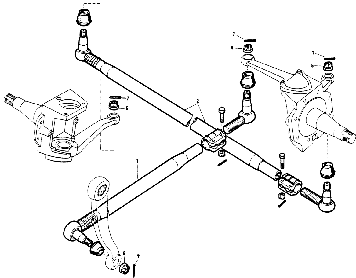
转向拉杆 (4×2, 6×2, 6×4)
